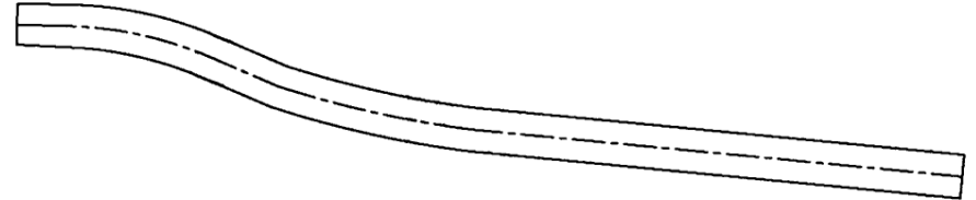
27x17 oval tapered to 16mm round single bend
